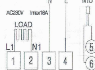
Electric heating wiring diagram
