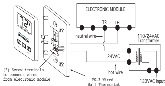
Figure #4 (Electronic Spark System)
