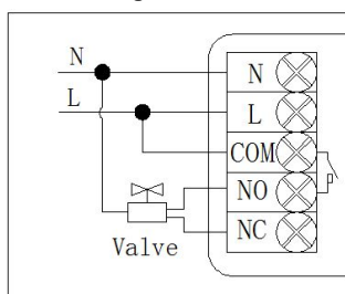
(2) Normal close valve
