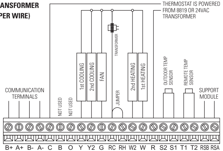
FIGURE 3 – Conventional Heat/Cool
