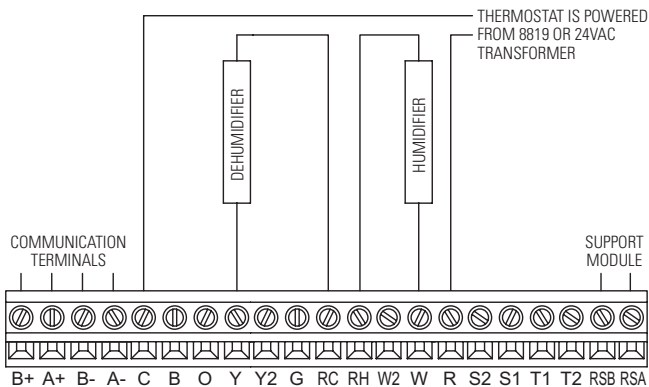
FIGURE 5 – Humidistat
