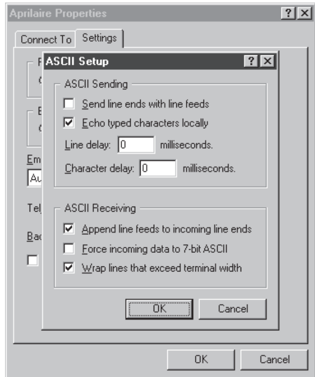
FIGURE 14 – ASCII Setup
