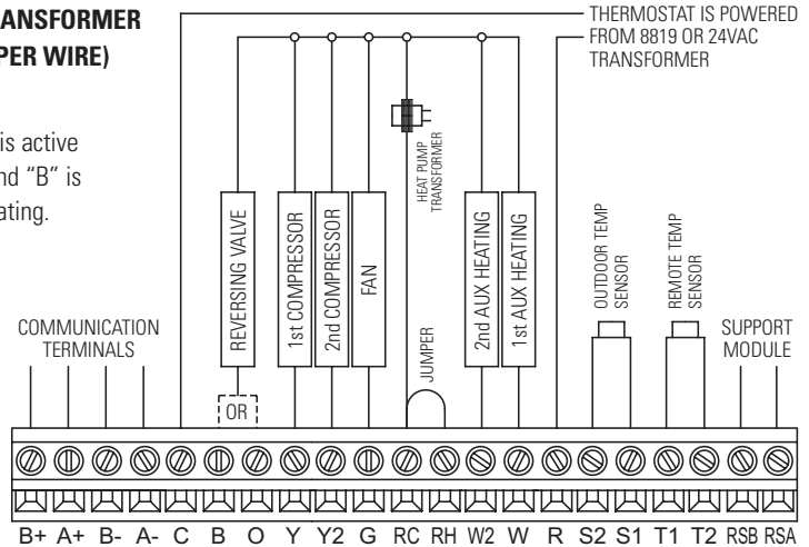
FIGURE 4 – Heat Pump
