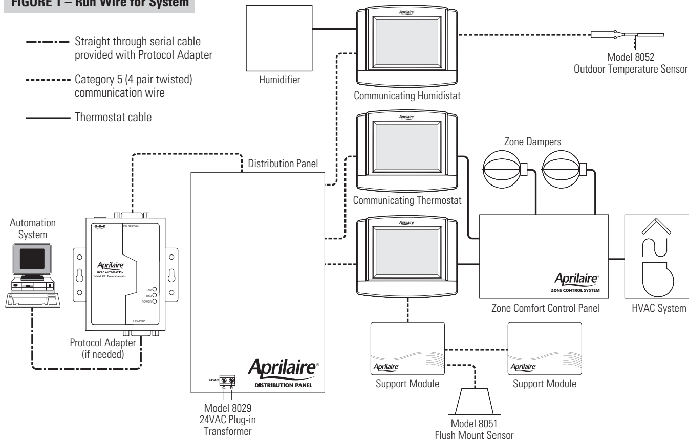
FIGURE 1 – Run Wire for System
