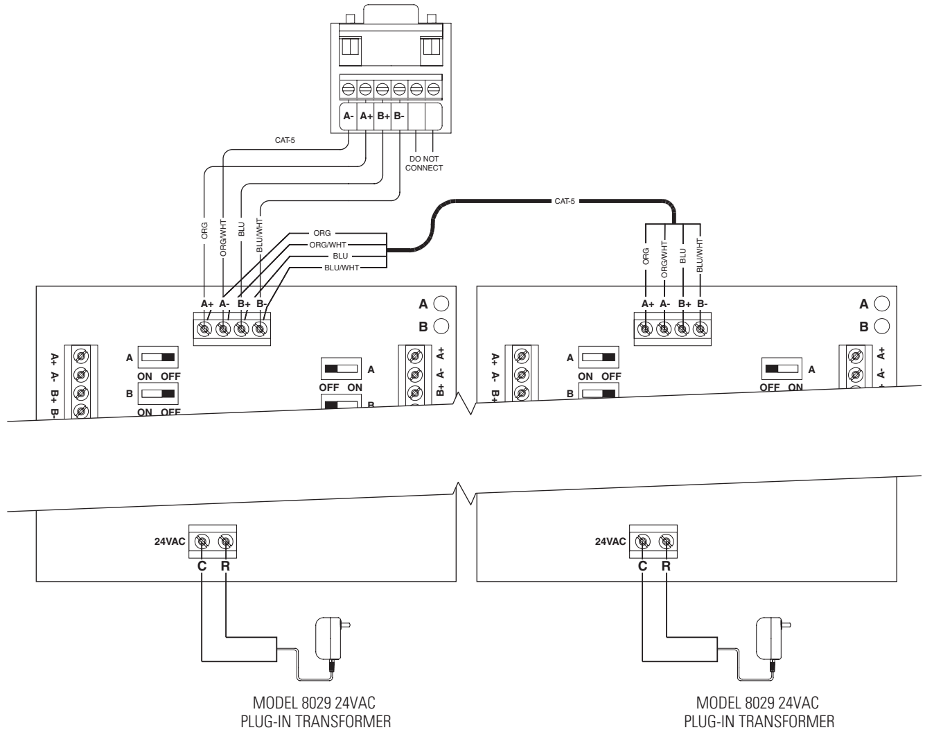
FIGURE 7 – Multiple Distribution Panels
