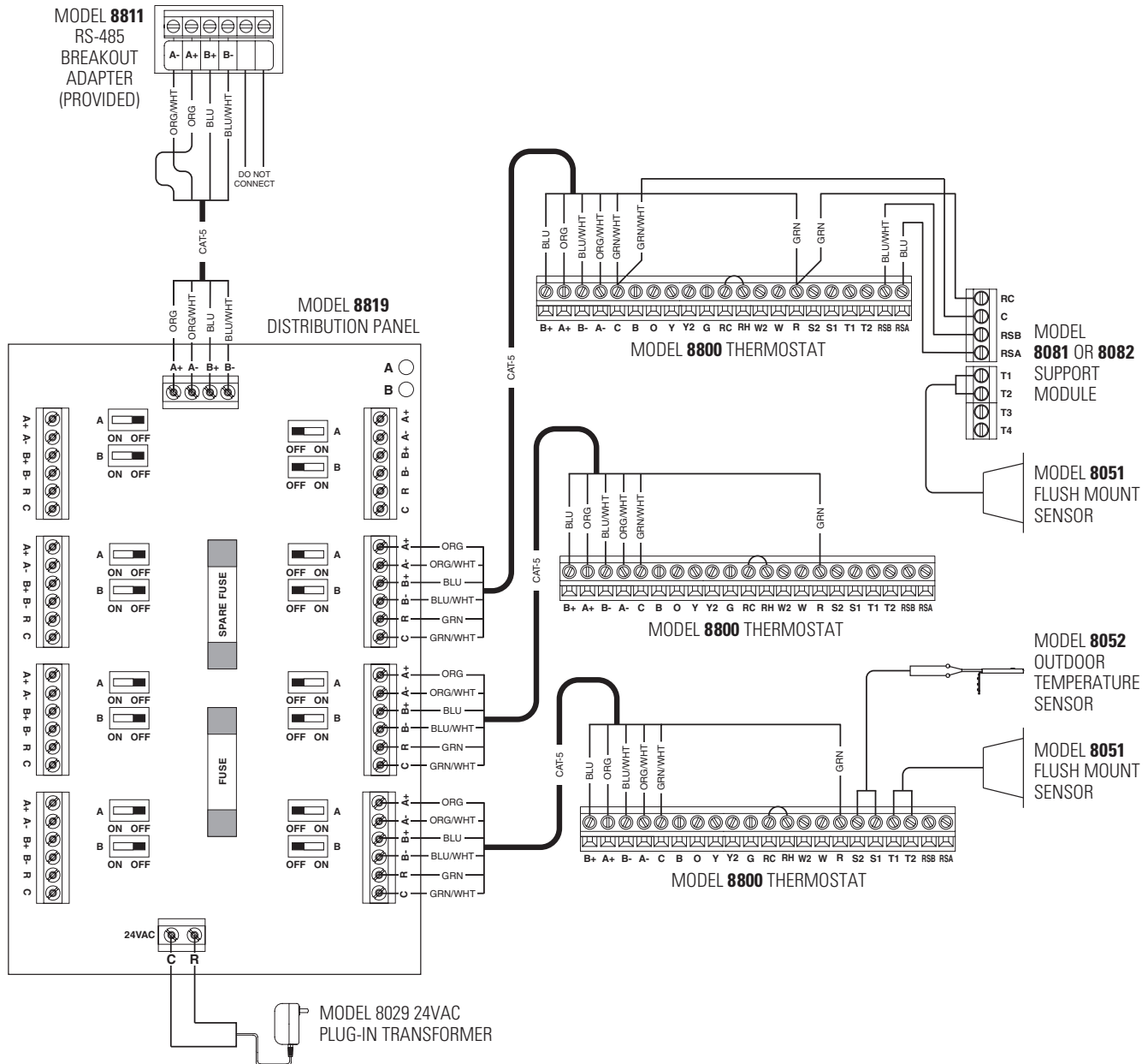
FIGURE 6 – System Communication Wiring
