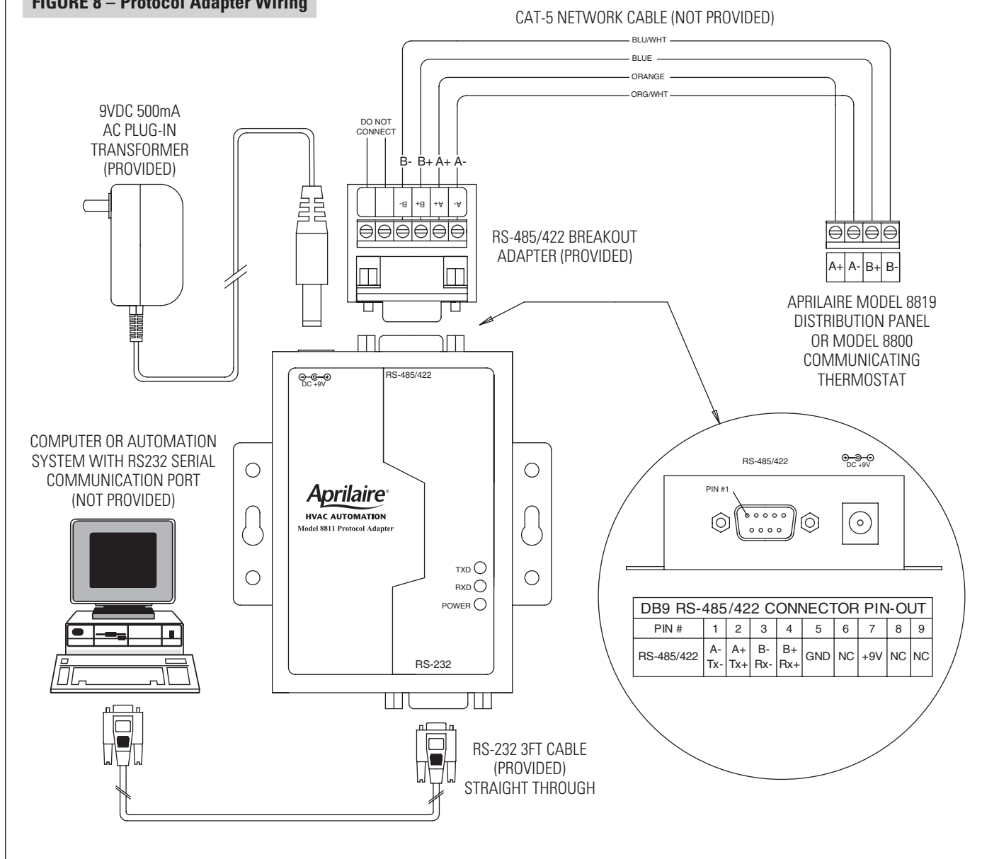
FIGURE 8 – Protocol Adapter Wiring
